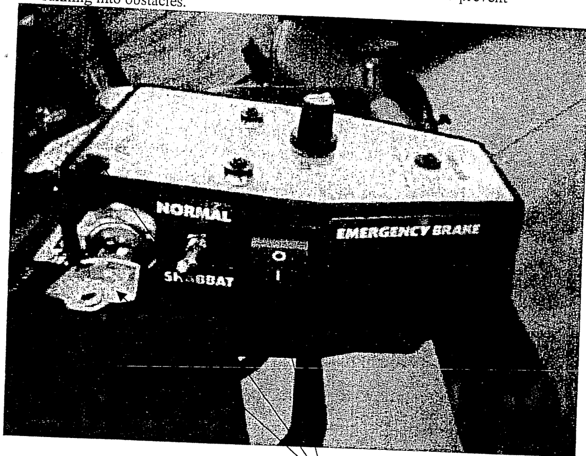
Shabbat Key Switch, Emergency Brake Switch, Shabbat LED
